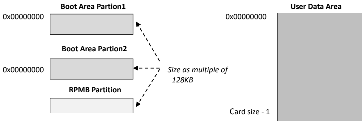
Figure 2 – e-MMC memory organization at time zero
